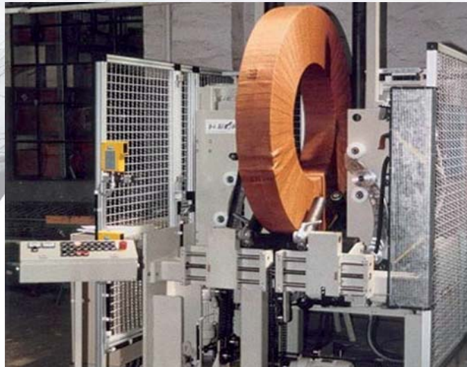
Fully automatic twist wrapping machine for ring-shaped products
